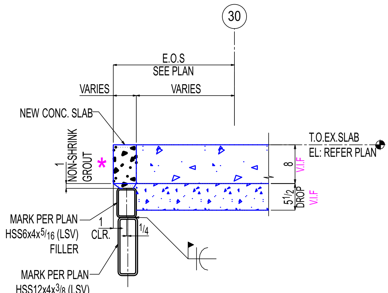
M-M E-12.00A (REF: 4/S315) OTHERS NOT SHOWN FOR CLARITY
