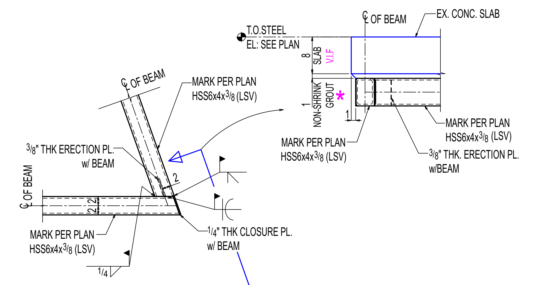
DETAIL-3 E-10.00 OTHERS NOT SHOWN FOR CLARITY
