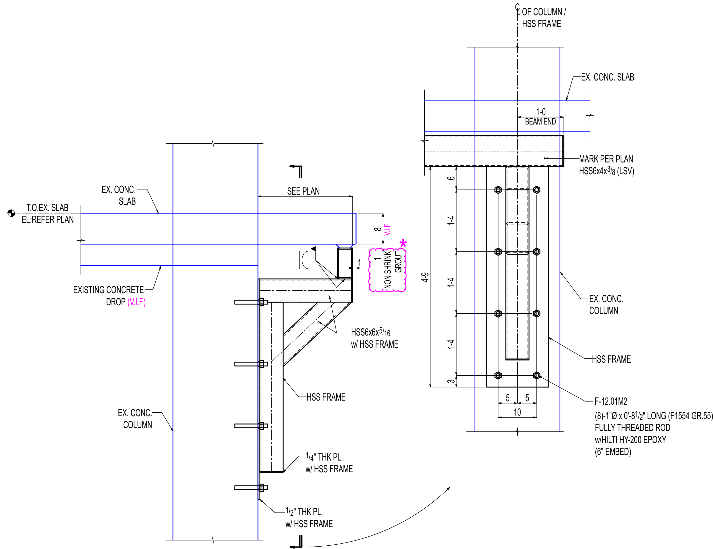
K-K E-12.00 (REF: 9/S315) (SIM) OTHERS NOT SHOWN FOR CLARITY
